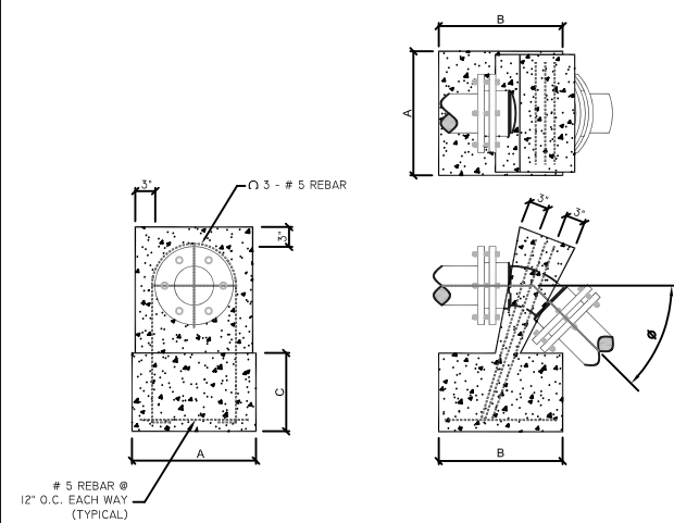
BLOCKING FOR 4"-10" GRAVITY BLOCKS
