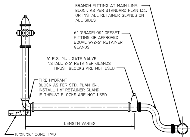
FIRE HYDRANT TYPICAL INSTALLATION TYPE 2
