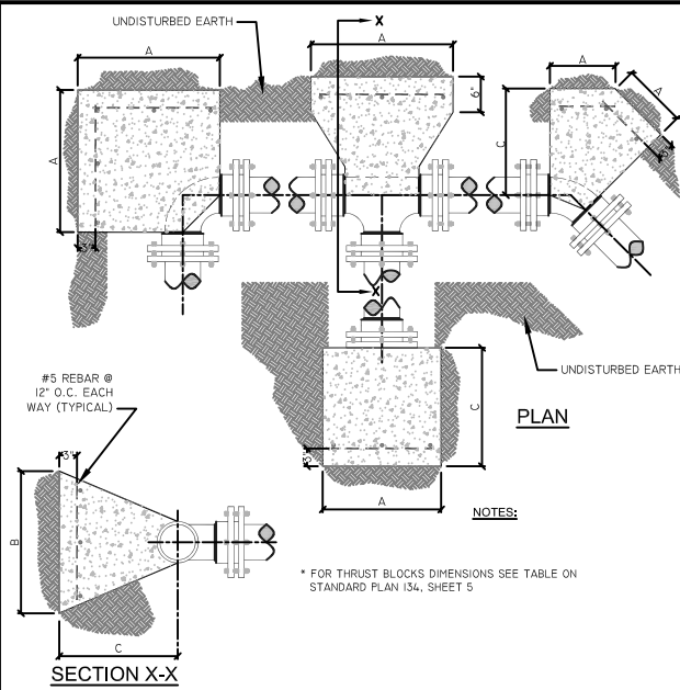
HORIZONTAL BLOCKING FOR FITTINGS
