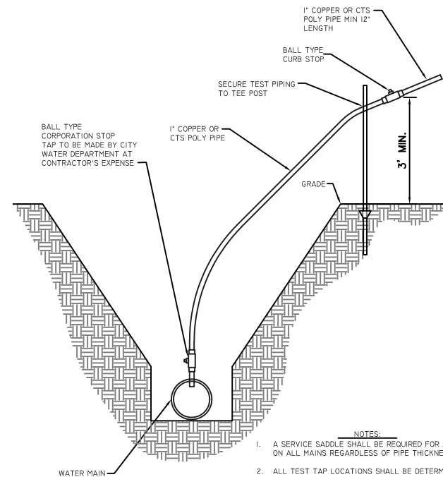
WATER MAIN TESTING & SAMPLING TAP
